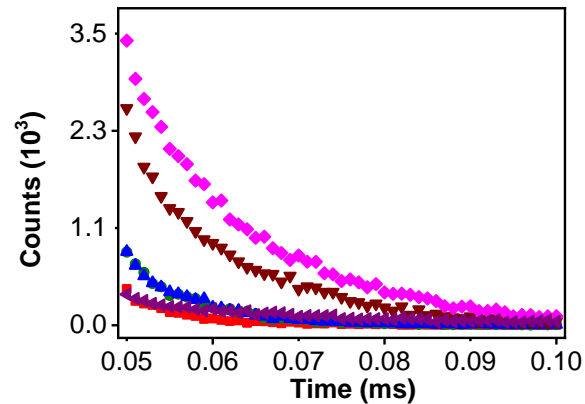
TCSPC recorded for studied samples
