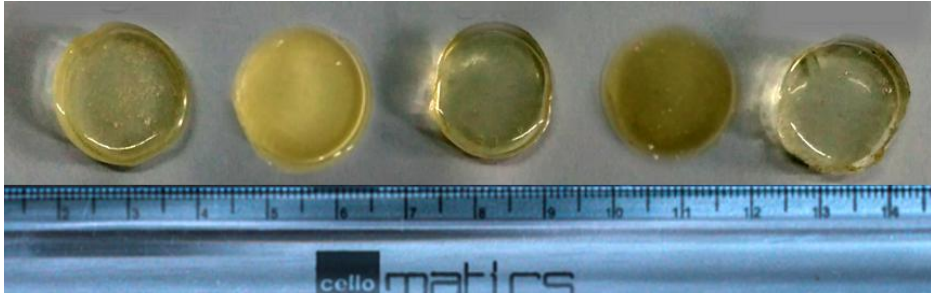
Glass samples fabricated by Sol-gel technique
