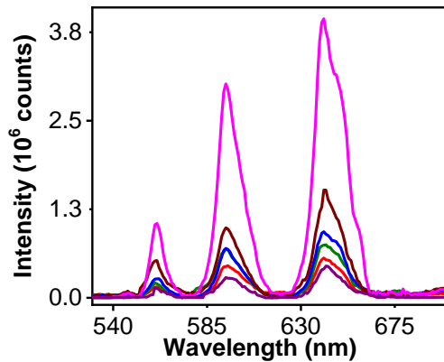
Photoluminescence spectra recorded for studied samples
