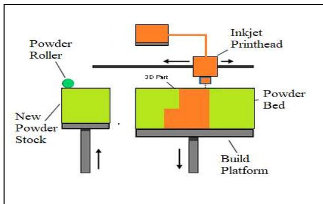
Fig. 3: Basic diagram of Binder Jetting equipment.
