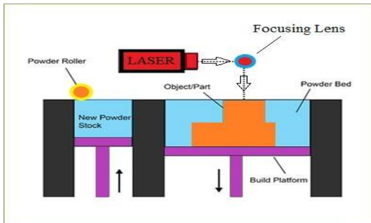
Fig. 7: Basic diagram of Powder bed fusion equipment.
