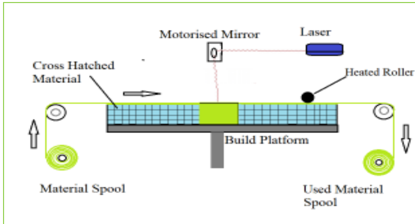
Fig. 5: Basic diagram of Sheet Lamination equipment.
