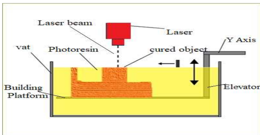
Fig. 6: Basic diagram of Vat Photopolymerization equipment.
