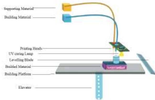
Fig. 2: Basic diagram of Material jetting equipment
